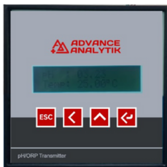
VIZ CLASSIC - pH/ORP ( Single Channel Transmitter with HART )
